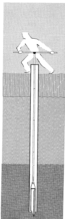
Lepelboor
